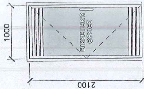
D-1 2100 X 1000mm ALUMINUM DOOR JAMB 210 X 1.00mm POWDER COATED ALUMINUM FRAME HEAVY DUTY SPRING DOOR, GUM FRAME WITH FROSTED STICKERS AND THE COMPLETE ACCESSORIES 1 SET(S)
