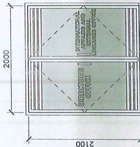
D-4 NOTE: EXISTING DOOR SUPPLY AND INSTALLATION OF FROSTED STICKERS 1 SET(S)
